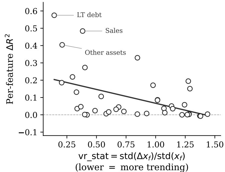
Ridge booster, L = 2 ( r = -0.45 )
